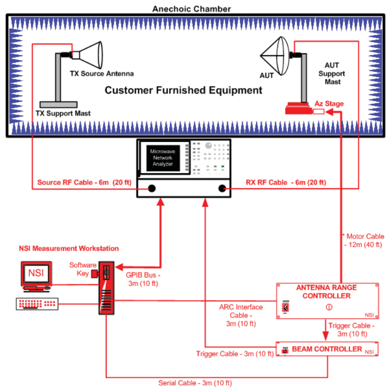
NSI-800F-10 Measurement System
